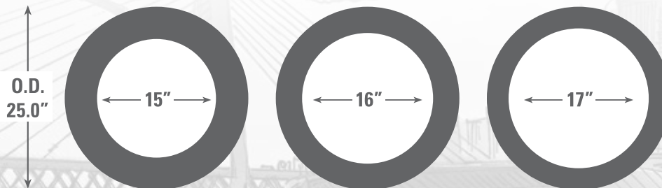
195/65R15 89V Original Size
